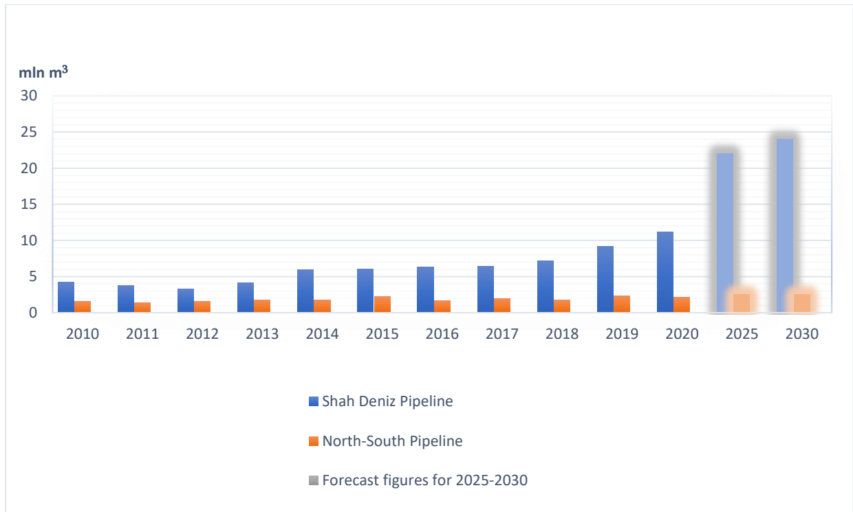
Figure 2 Transit of natural gas, mln m 3 a year
