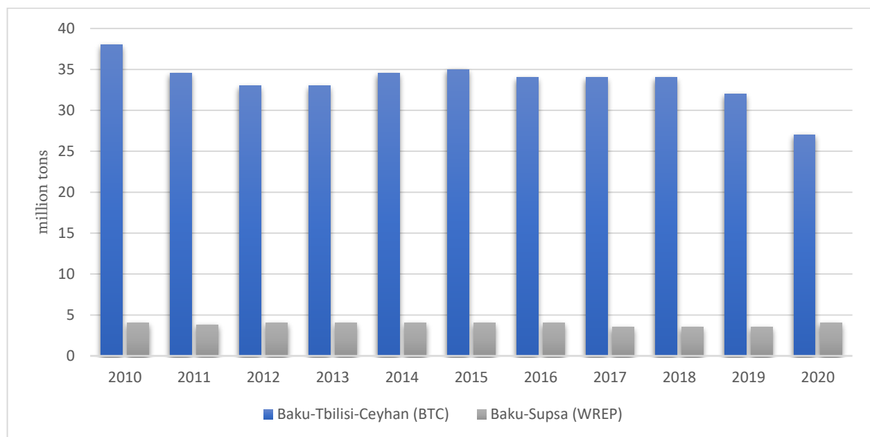
Figure 1 Load of Baku-Tbilisi-Ceyhan and Baku-Supsa pipelines in 2010-2020
