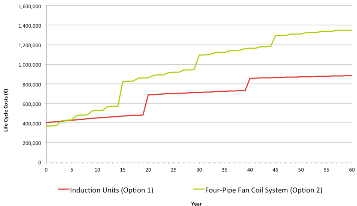
Figure 1: Component comparison - induction beams and Fancoil system
